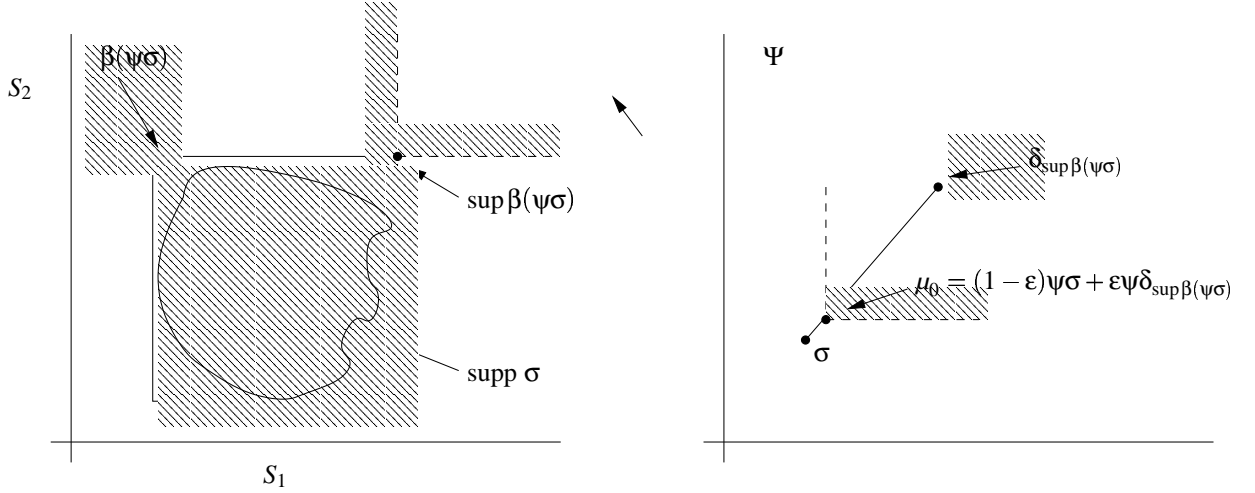
Figure 2: Unstable mixed equilibrium
